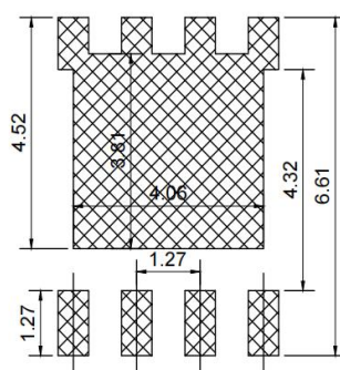
Land Pattern (Only for Reference)
